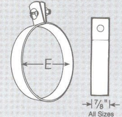
Tube Hanger
