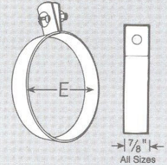
Tube Hanger
